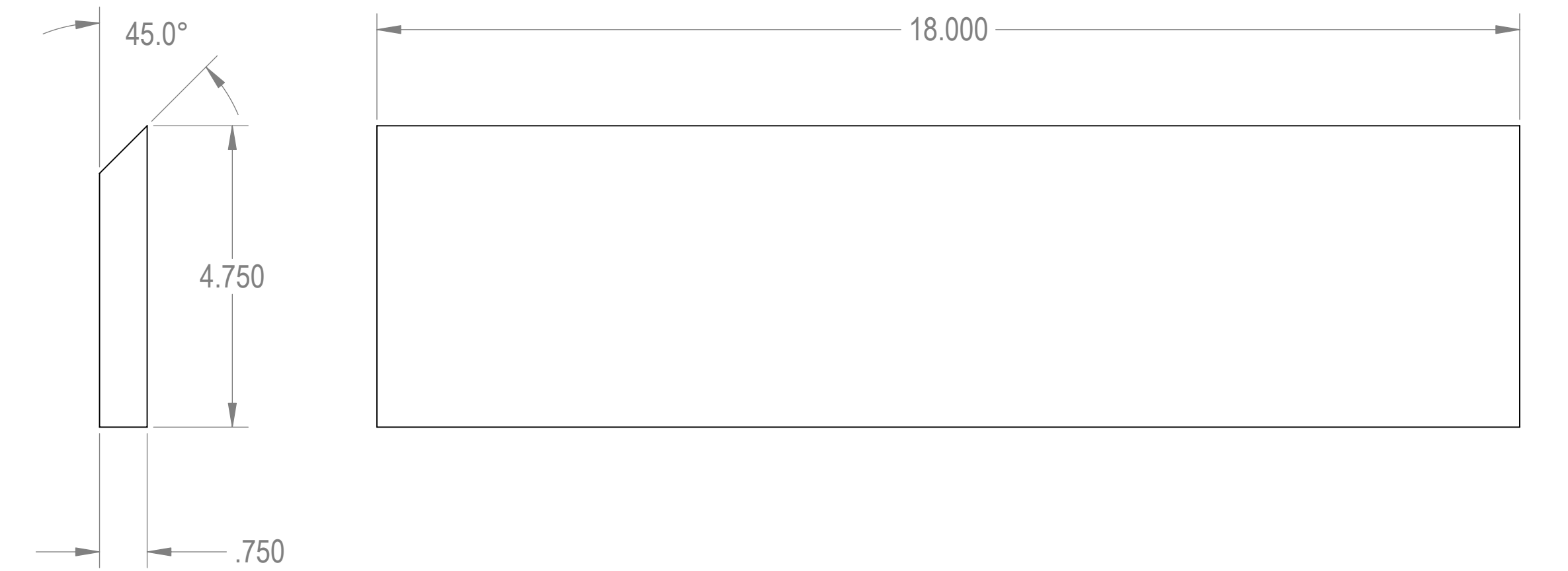
BOX FRONT RETAINER
