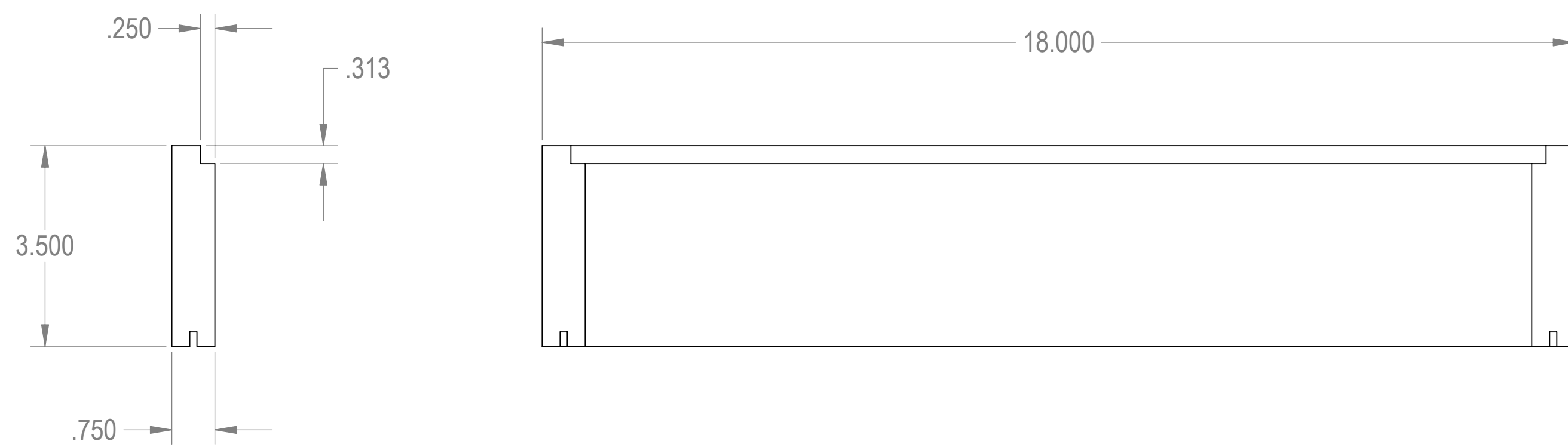
BOX SIDE
